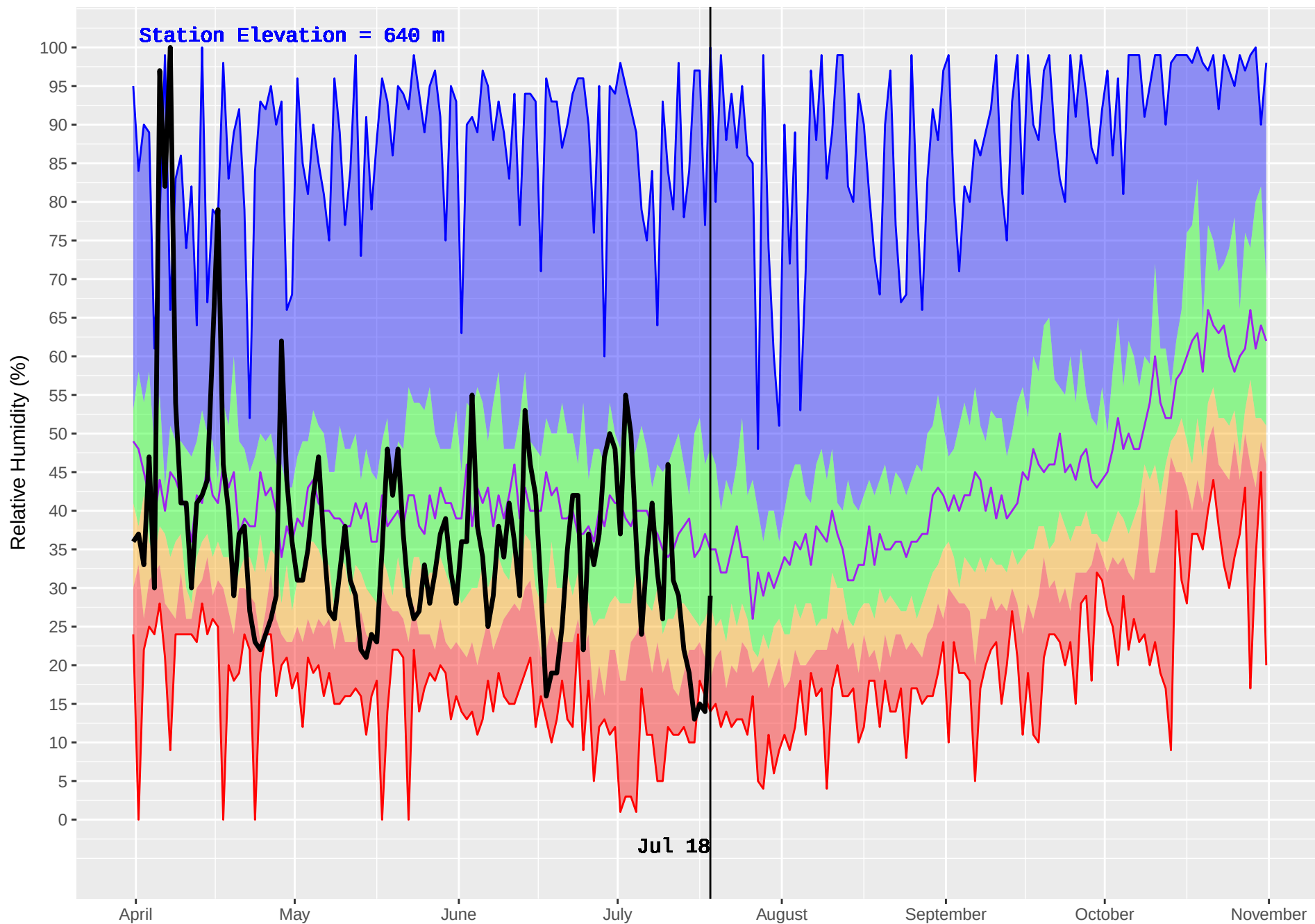
MERRITT HUB (294) : Historical (1978–2016) and Current (2018) Daily Relative Humidity
