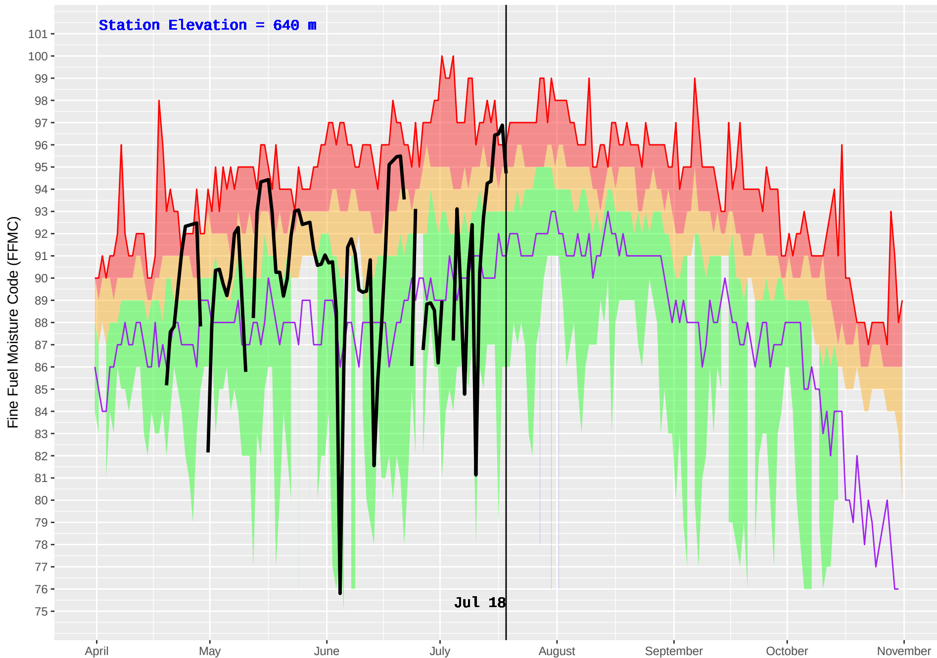
MERRITT HUB (294) : Historical (1978–2016) and Current (2018) Daily Fine Fuel Moisture Code (FFMC)
